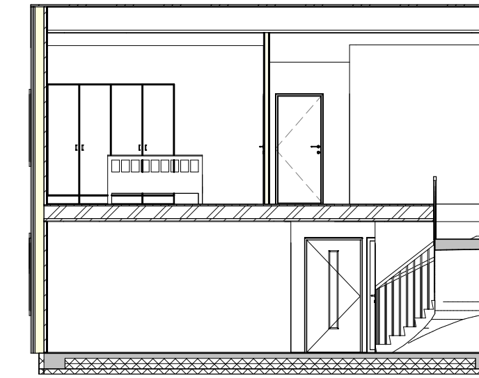
1 ÞVERSNID 1 : 100
